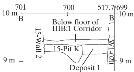
Fig. 82b. South of Building 1, section B-B; cf. Fig. 81.
