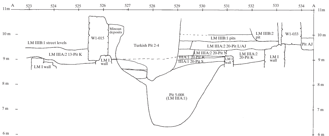
Fig. 54. Street and Rubbish Area Southeast, section A-A; cf. Fig. 53. Reproduced 67% of original in 1:50.
